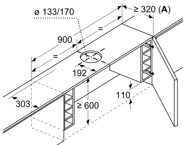
measurements in mm Fitting the telescopic hood with lowering frame
