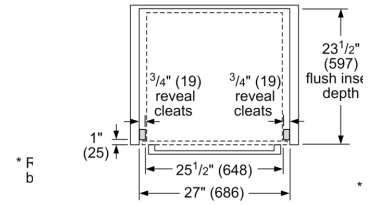
Flush Install Top View
