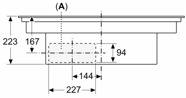
measurements in mm Front view
