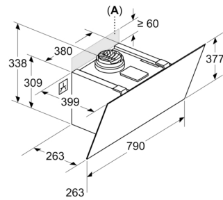
Measurements in mm Appliance in circulated air mode without duct
