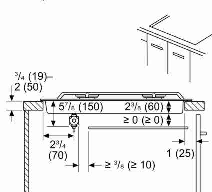
Measurements in inches (mm) Cooktop over door
