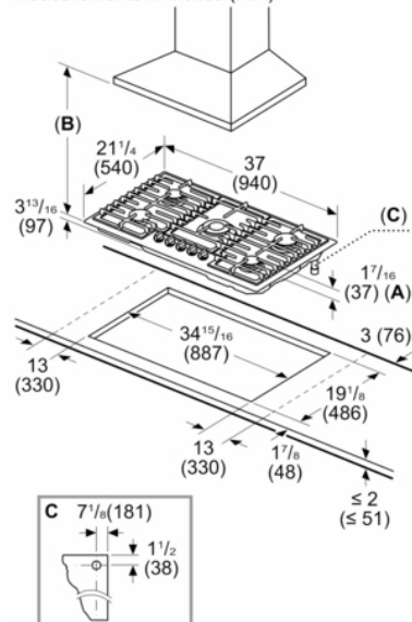
Measurements in inches (mm) Cooktop over oven
