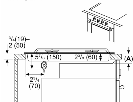
Measurements in inches (mm) Cooktop over oven
