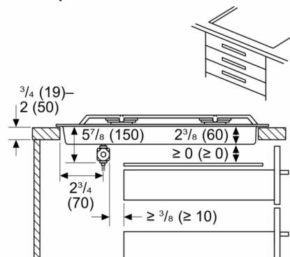
Measurements in inches (mm) Cooktop over drawer
