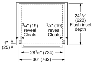
Flush installation Top view
