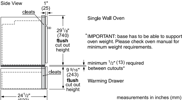
Flush Installation Single Oven over Warming Drawer
