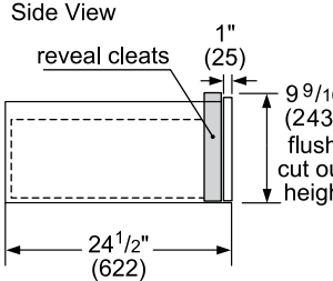
30" & 27" Flush Installation
