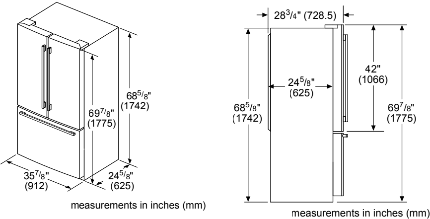
36" Freestanding Dimensions
