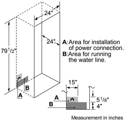
24" B11CB81SSS Installation
