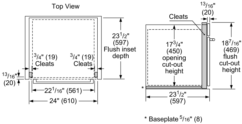
Flush Installation
