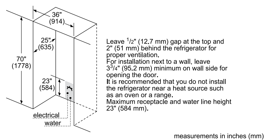
36" Freestanding Installation
