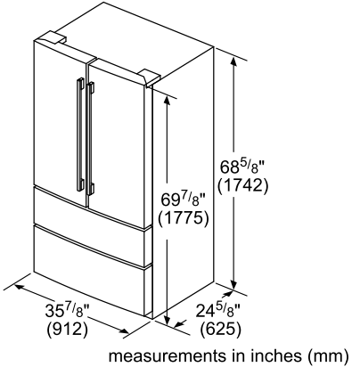
36" Freestanding Dimensions
