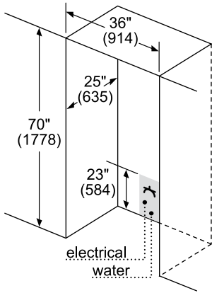
36" Freestanding Installation
