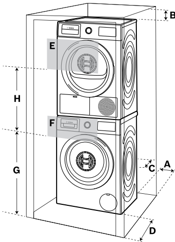
Enclosure Dimensions
