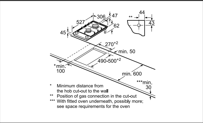
PRB326B70E Measurements in mm
