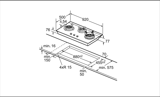
PBD9331MS Measurements in mm
