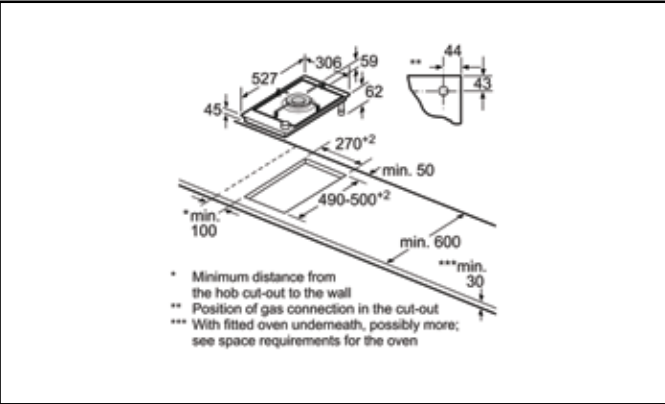
PRA326B70E Measurements in mm
