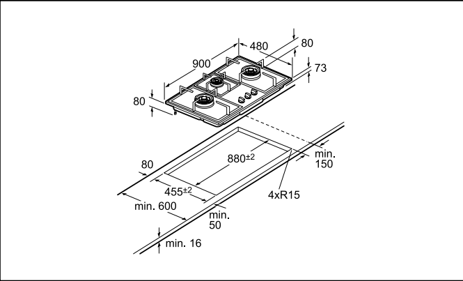
PBD9351MS Measurements in mm
