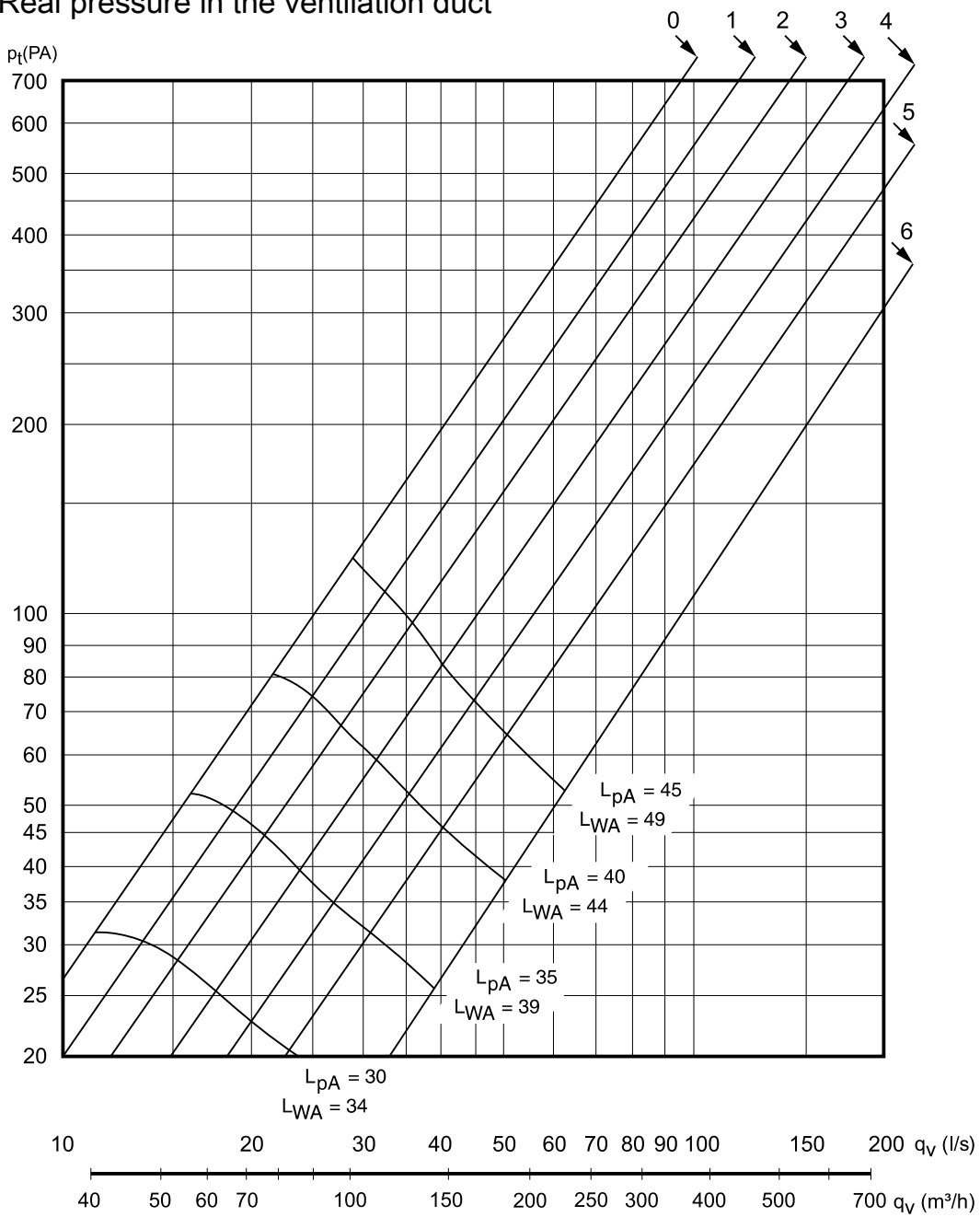
Real pressure in the ventilation duct
