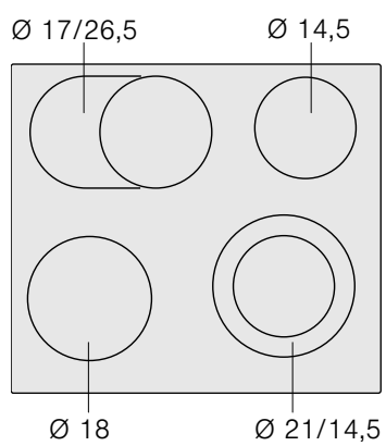
NKN6..BA..
