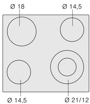
NKN6..BA..
