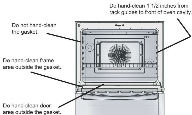
Figure 13: Cleaning Guidelines
