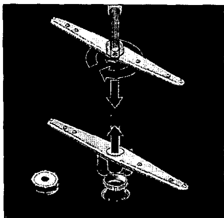
Spray arms
