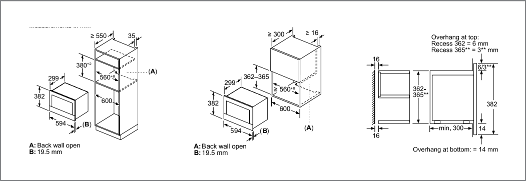
Microwaves BFL7221B1B
