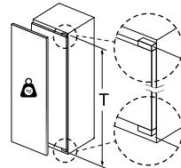
Maximal permissible weight of the unit fronts
