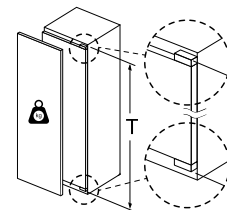
Maximal permissible weight of the unit fronts
