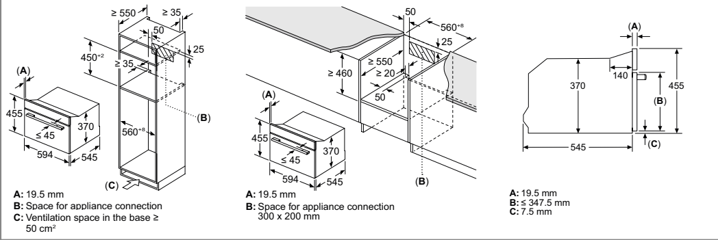
Compact Microwave CEG732XB1B
