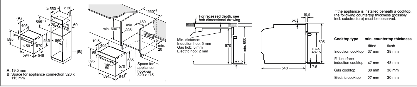
Single ovens HRS574BS0B, HBS573BS0B, HBS573BB0B, HRS534BS0B, HBS534BS0B, HBS534BB0B, HBS534BW0B
