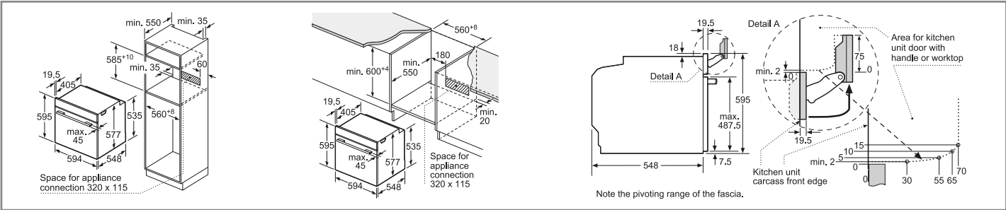
Single ovens HRG7764B1B, HSG7364B1B
