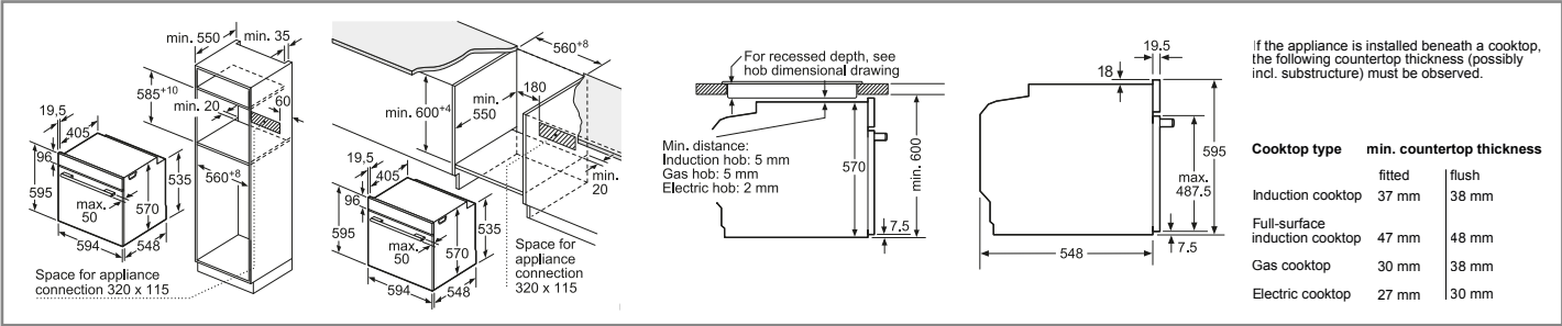
Single ovens HMG7764B1B, HBG7764B1B, HBG7741B1B, HBG7341B1B
