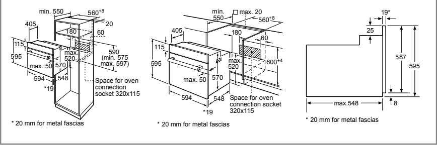
Series 2 single ovens HHF113BR0B, HHF113BA0B
