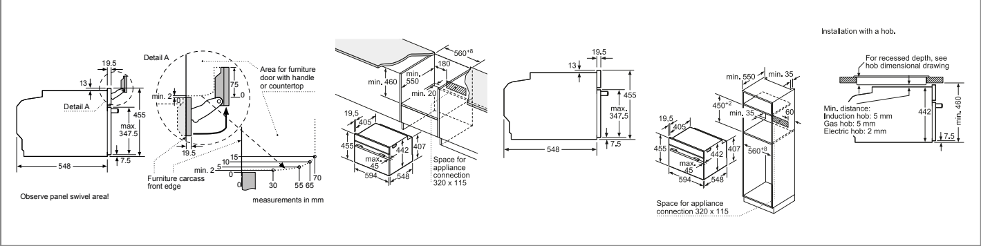
Compact oven (with added steam) CSG7584B1, CSG7361B1 Compact ovens (with microwave) CMG7761B1B, CMG7361B1B, CMG7241B1B
