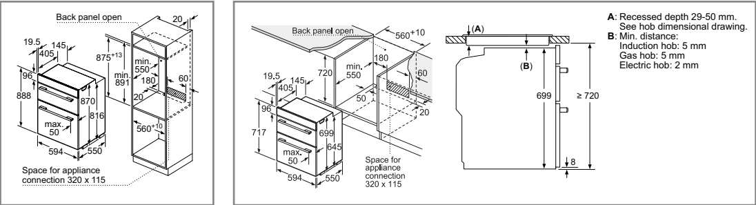
Built-in double ovens MBA5785S6B, MBS533BS0B, MBS533BB0B, MHA133BR0B Built-under double ovens NBS533BS0B, NBS533BB0B
