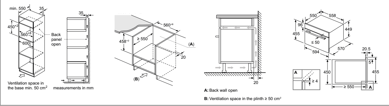
Compact Combination Microwave Ovens CMA583MS0B, CMA583MB0B
