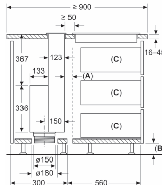
Measurements in mm Standard, top-mounted installation
