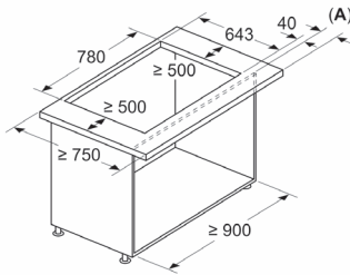
Measurements in mm Combination with electric hob Seamless, top-mounted installation
