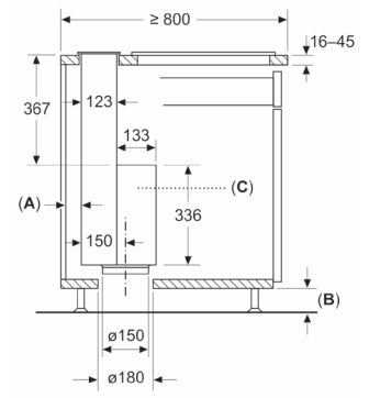
Measurements in mm Standard, top-mounted installation
