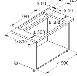
Measurements in mm Combination with electric hob Standard, top-mounted installation
