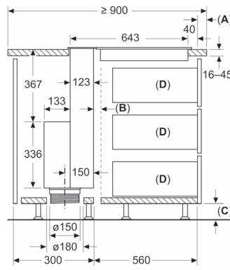
Measurements in mm Seamless, top-mounted installation (Special accessory required)
