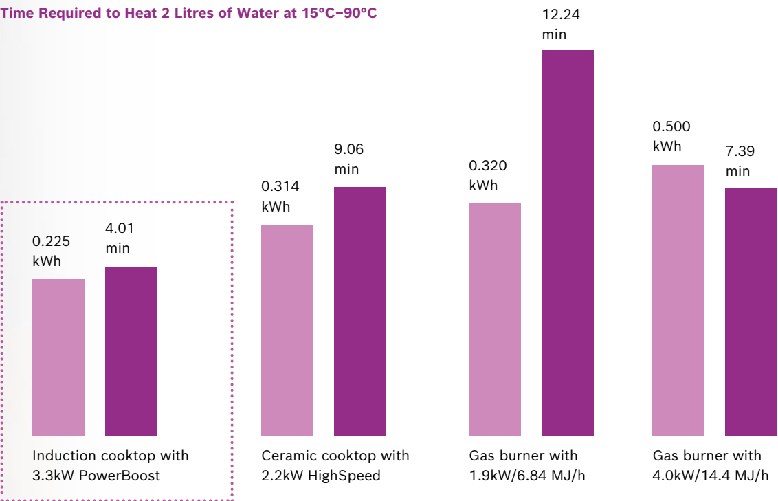
Time Required to Heat 2 Litres of Water at 15°C–90°C
