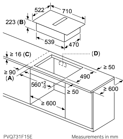
PVQ731F15E Measurements in mm
