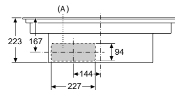
PVQ731F15E, PVQ811F15E Measurements in mm
