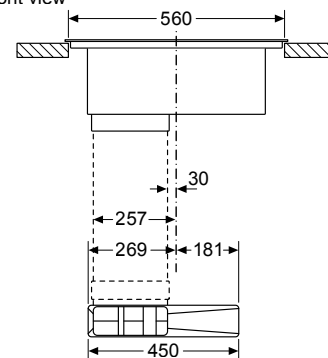
PVQ731F15E Measurements in mm
