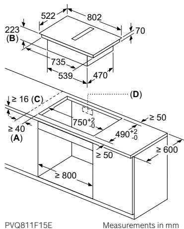
PVQ811F15E Measurements in mm
