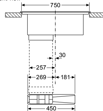
PVQ811F15E Measurements in mm
