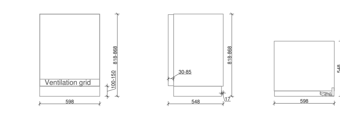
BOSCH GUD15AFF0G
