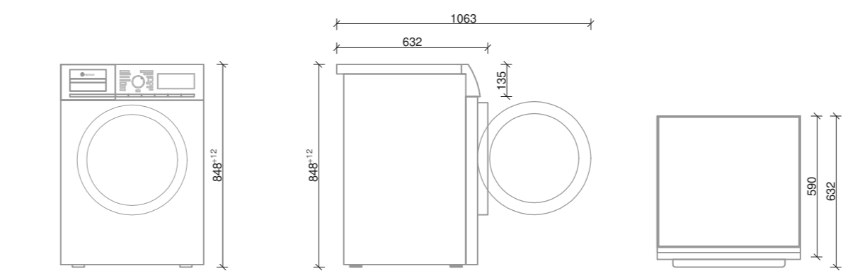
BOSCH WGA244BGHK
