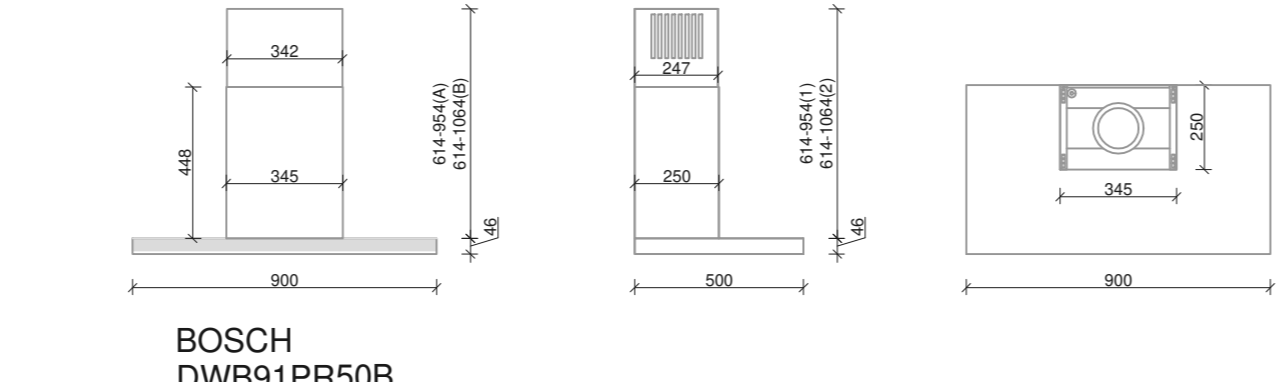
BOSCH DWB91PR50B
