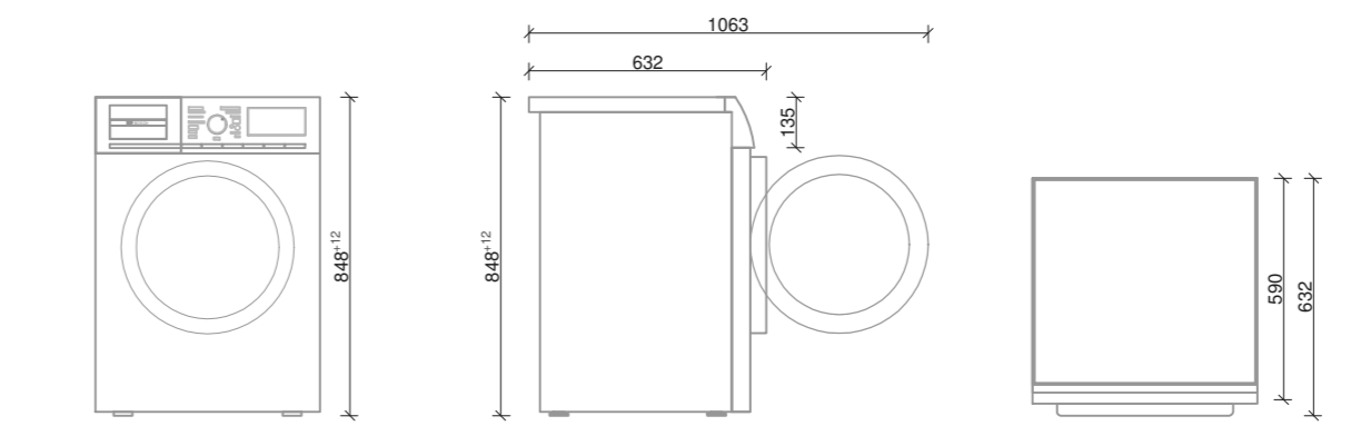
BOSCH WGA256BGHK
