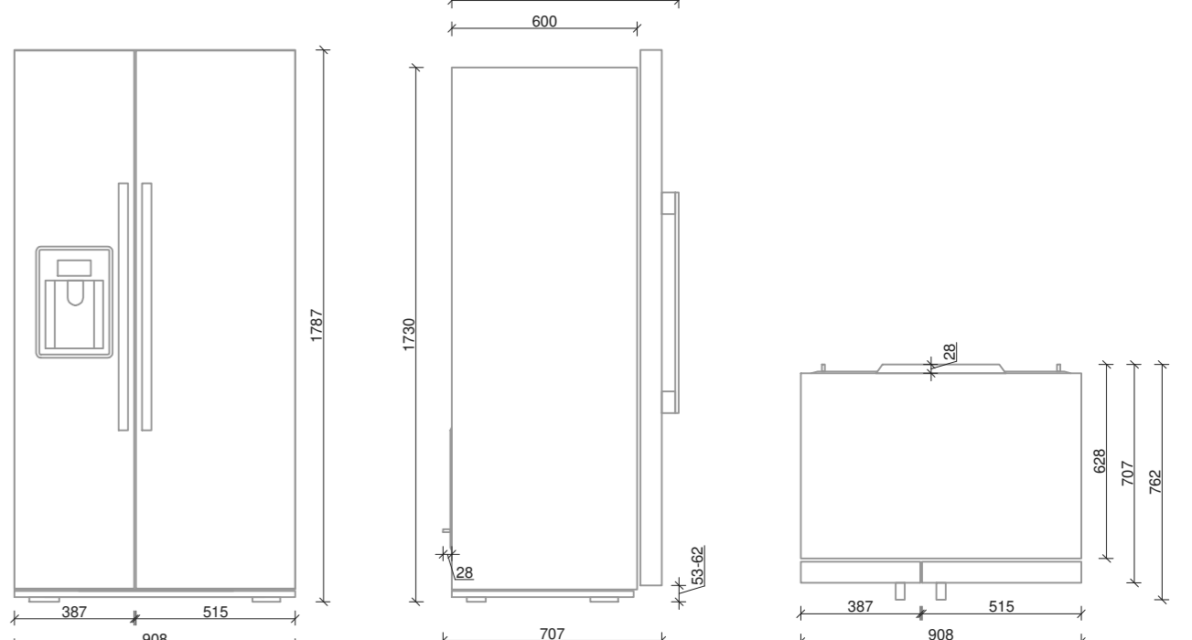
BOSCH KAI93VIFPG
