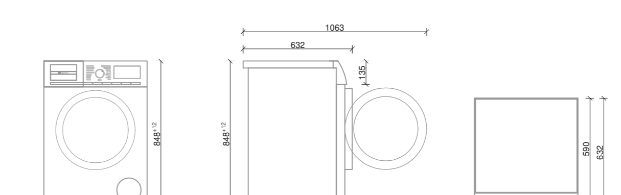
BOSCH WGA246UGHK
