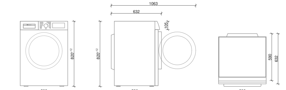
BOSCH WUU2846BHK
