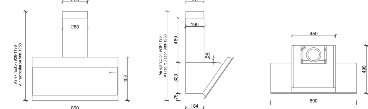
BOSCH DWK98JQ66
