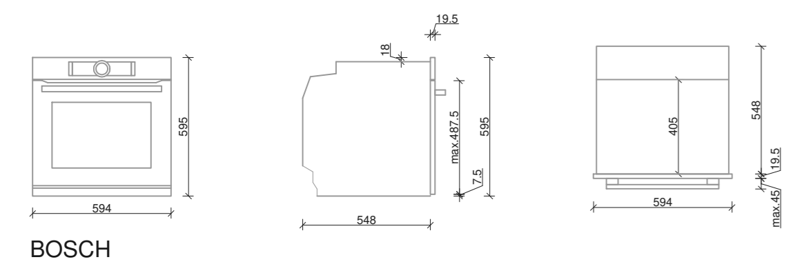
BOSCH HBG633BS1
