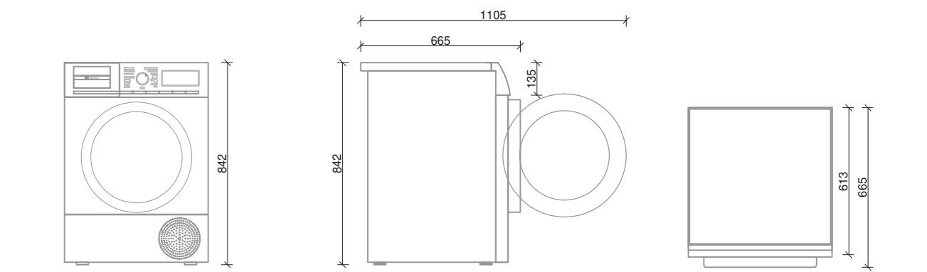
BOSCH WTX87MH0SG
