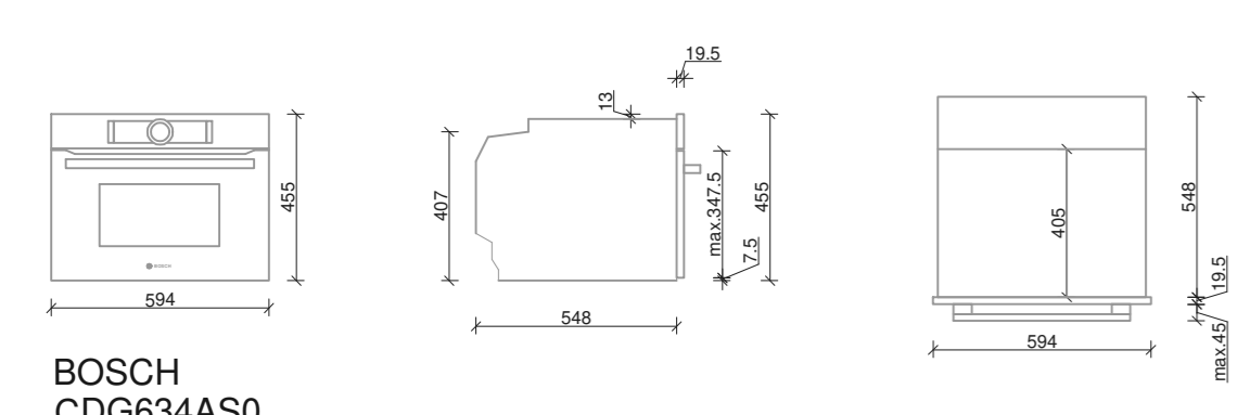
BOSCH CDG634AS0
