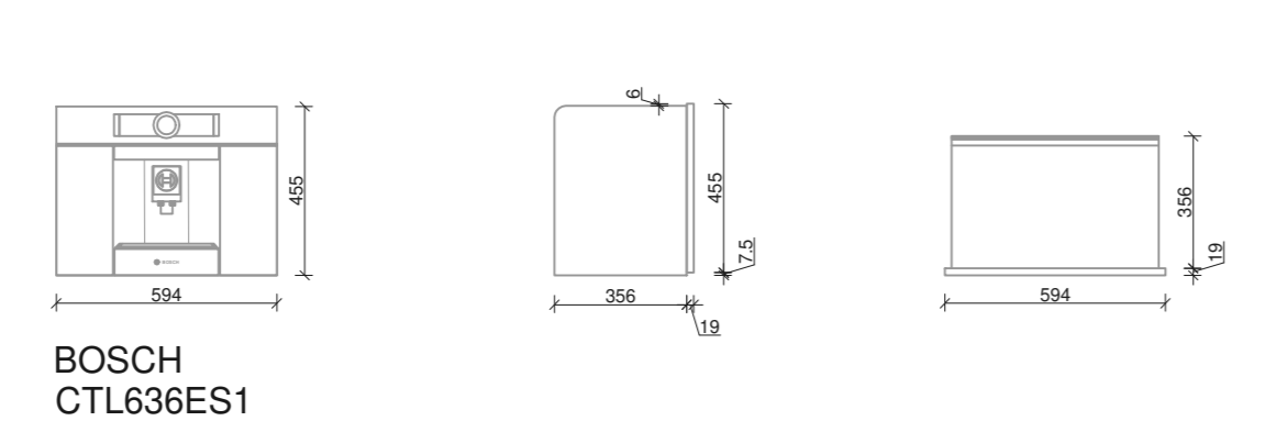
BOSCH CTL636ES1
