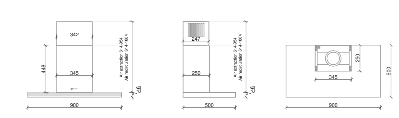
BOSCH DWB98PR50
