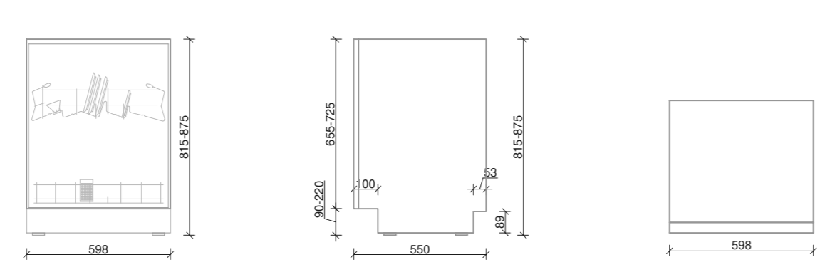
BOSCH SMD6ZCX50E
