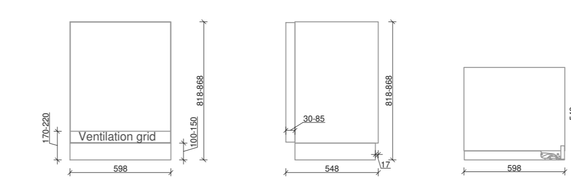
BOSCH KUL15AFF0G
