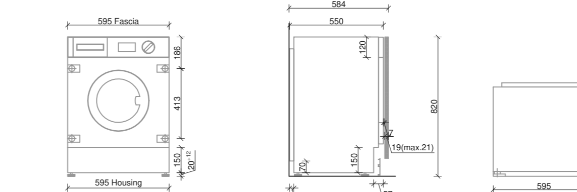
BOSCH WKD28351HK
