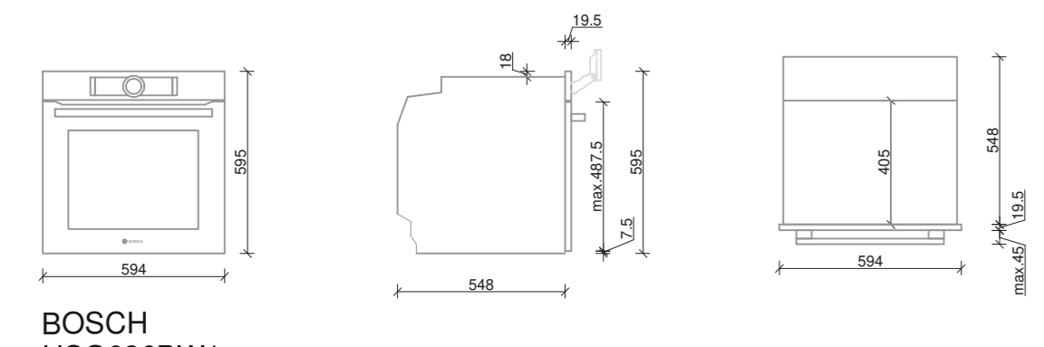
BOSCH HSG636BW1
