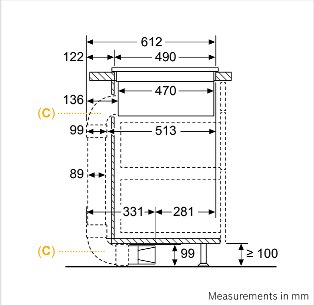
With HZ9VDSB2 (top) Vertical 90° "L" bow flat duct element (male).
