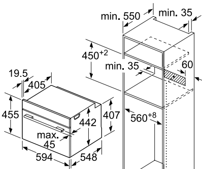
Space for appliance connection 320 x 115
