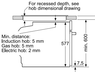
Installation with a hob.
