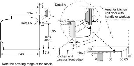
Note the pivoting range of the fascia.
