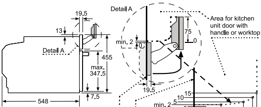
Note the pivoting range of the fascia.
