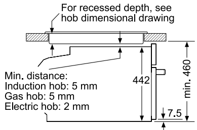
Installation with a hob.
