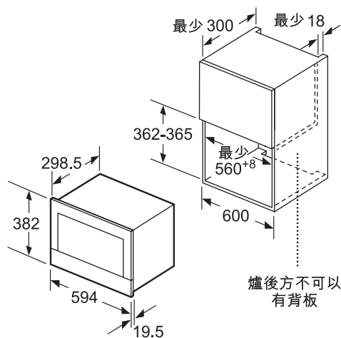
微波爐設於吊櫃
