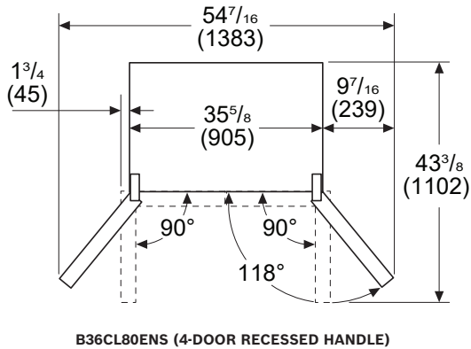
B36CL80ENS (4-DOOR RECESSED HANDLE)
