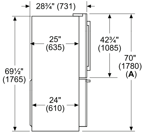
(A) Add ⅝" (17) with front leveling feet fully extended.
