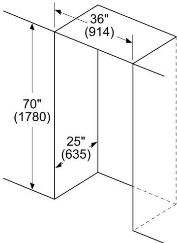
Leave ½" (12.7) gap at the top and 1" (25.4) behind the refrigerator for proper ventilation. It is recommended that you do not install the refrigerator near a heat source such as an oven or a range.
