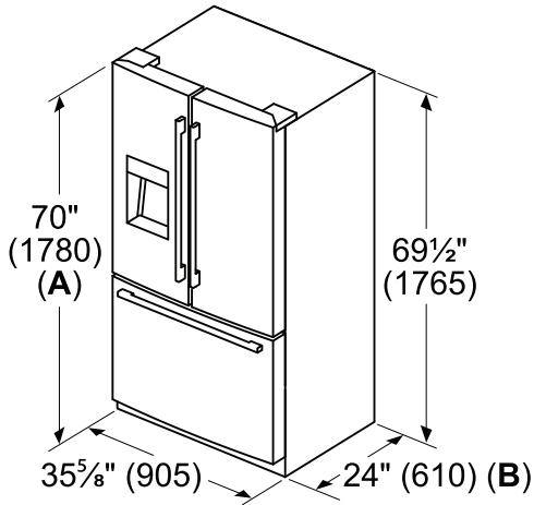
(A) Add ⅝" (17) with front leveling feet fully extended. (B) Add 1" (25) for fixed spacers on back.
