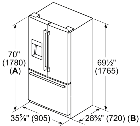
(A) Add ⅝" (17) with front leveling feet fully extended. (B) Add 1" (25) for fixed spacers on back.
