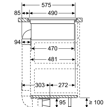
measurements in mm Side view
