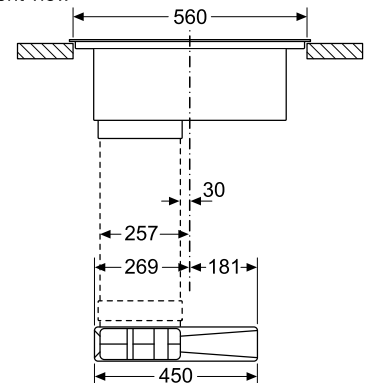
measurements in mm Front view
