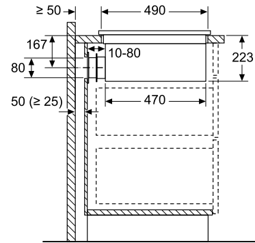
measurements in mm Side view
