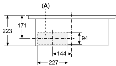
measurements in mm Front view
