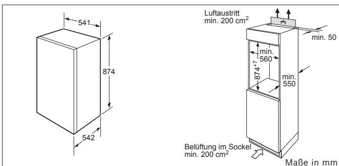
KIL18V60 | KIR18V60 | KIR18V51
