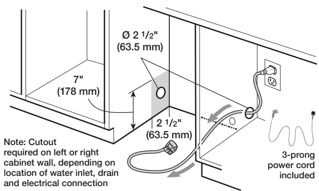
Example of an Electrical Receptacle Installation
