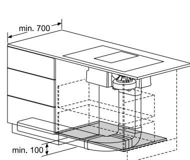
PVS851F21E with HEZ381401 Ducted extraction kit
