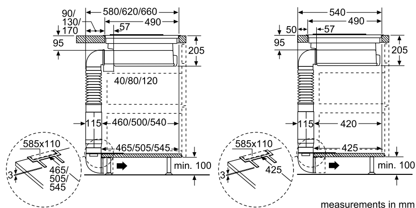
PVS851F21E with HEZ381501 Recirculation extraction kit
