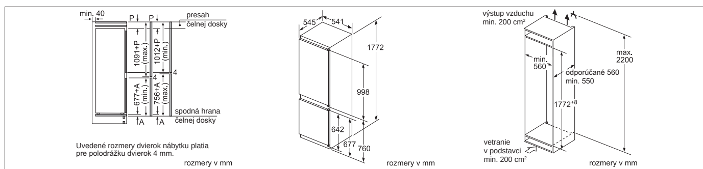
KIV 86VS30
