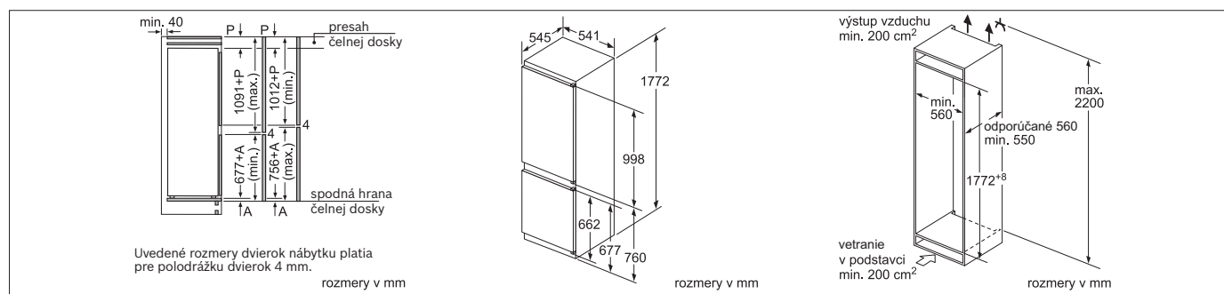
KIN 86VS30
