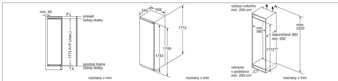
KIL 82AF30
