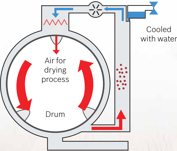
Traditional Water Condensation Technology
