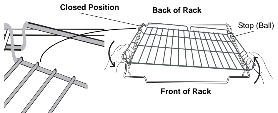
Figure 5: Reassembly
