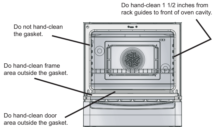
Figure 17: Cleaning Guidelines
