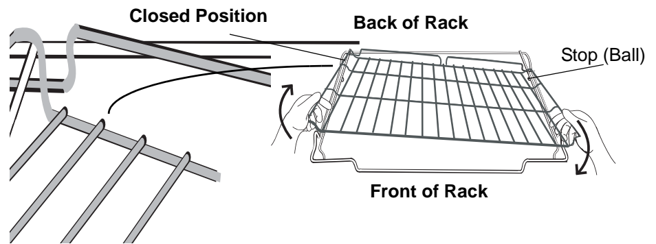
Figure 4: Disassembly
