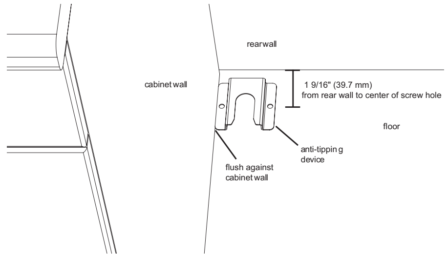
Figure 5: Anti-Tip Bracket
