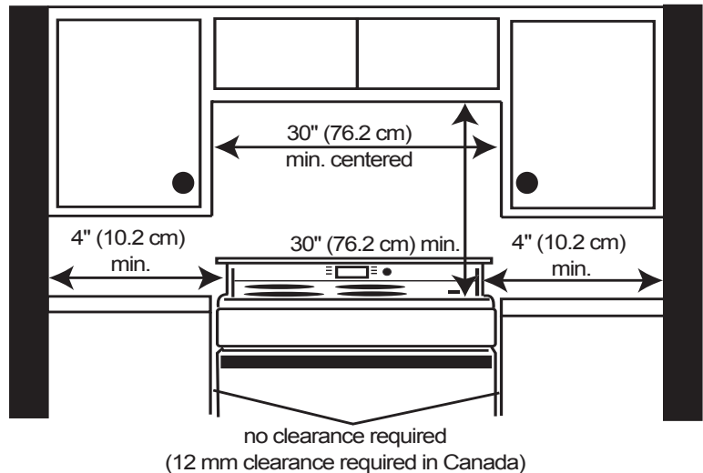
Figure 4: Cabinet Preparation
