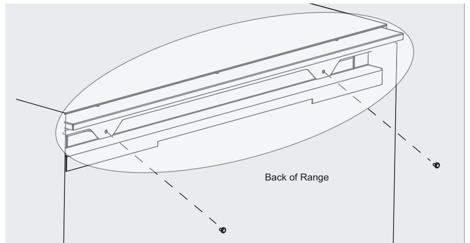
Figure 7: Install Backwall Trim Strip
