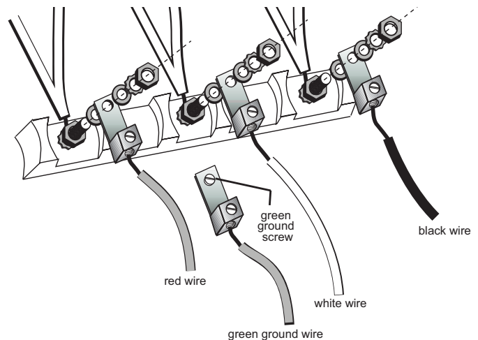
Figure 18: Completed Four Wire Flexible Conduit Connection
