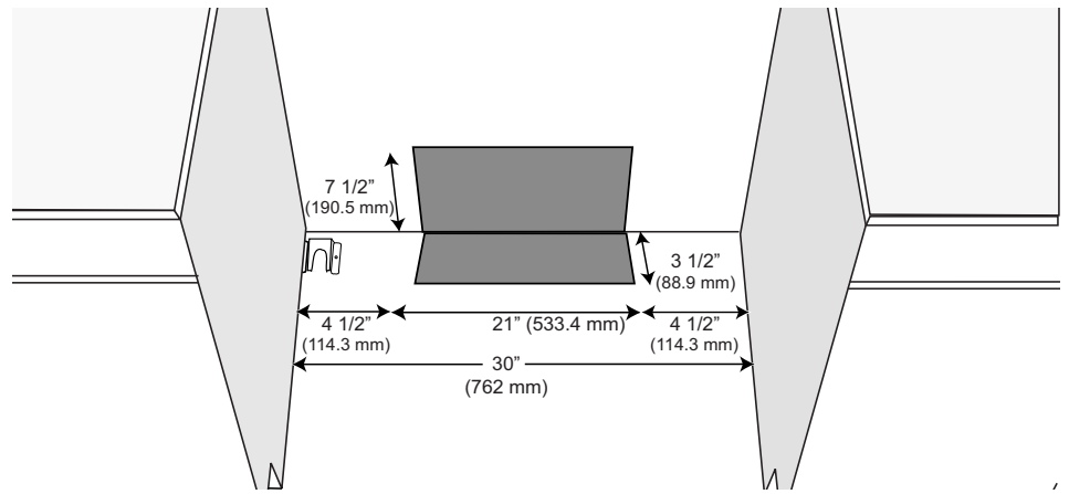
Figure 1: Cooktop Clearances
