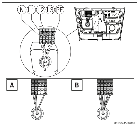
Bild 493 Elanslutning A = 1-fasininstallation B = 3-fasininstallation
