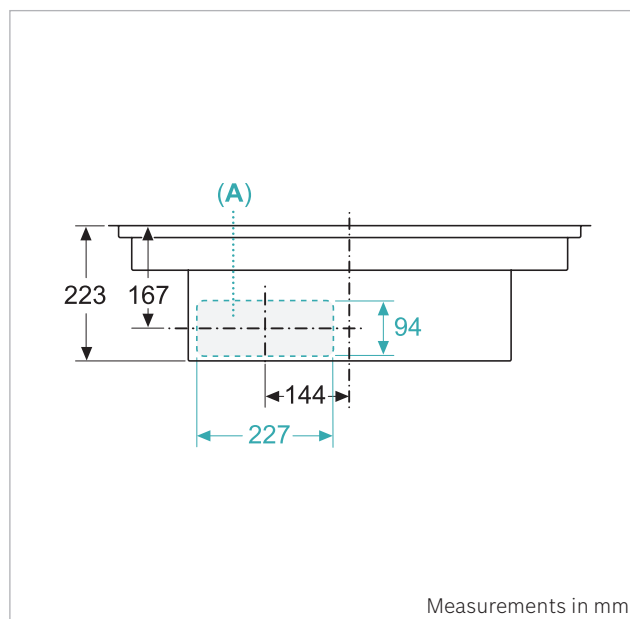
Cooktop with integrated ventilation module variants for top-mounted plannings PXX895D66E | PVQ895F25E | PIE895B15E
