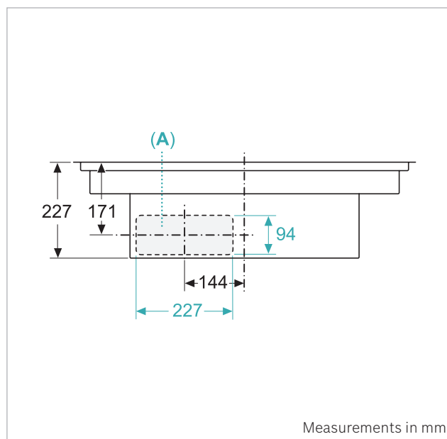
Cooktop with integrated ventilation module variants for flush-mounted plannings PXX821D66E | PVQ821F25E
